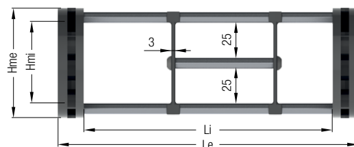
Type A (with horizontal separators not in full width)
