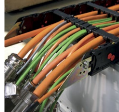
Program LC55: Wired with cables and connectors
